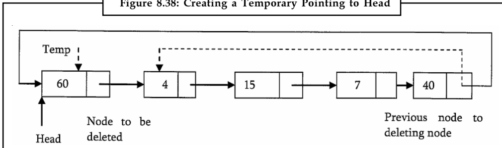
Figure 8.38: Creating a Temporary Pointing to Head
