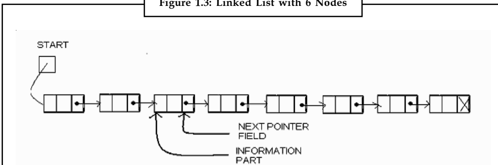
Figure 1.3: Linked List with 6 Nodes
