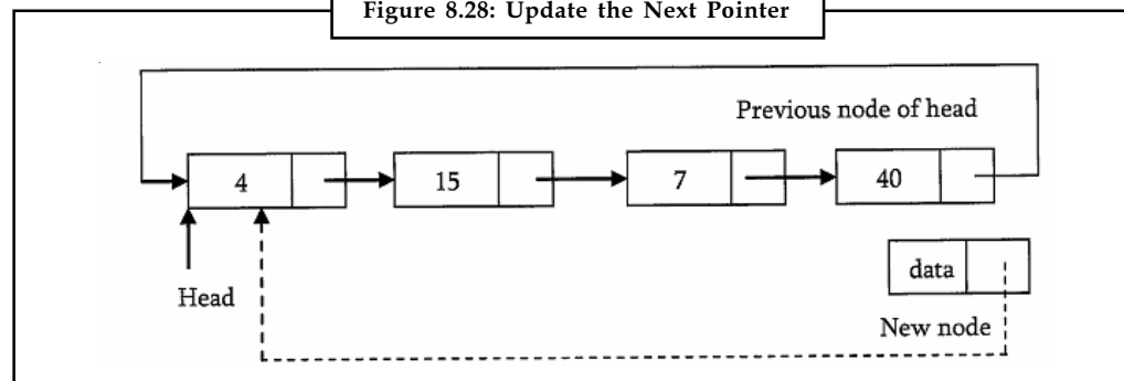
Figure 8.28: Update the Next Pointer
