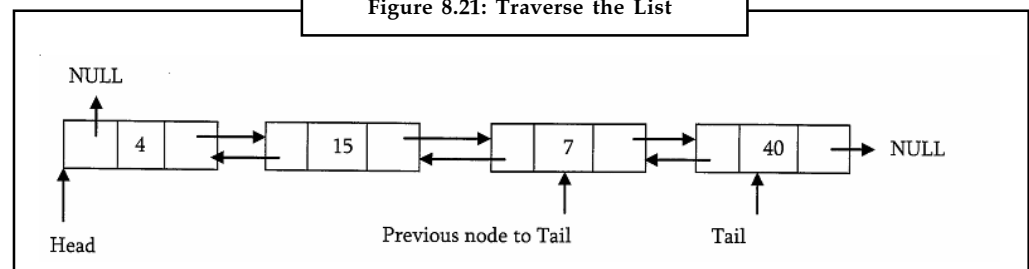
Figure 8.21: Traverse the List
