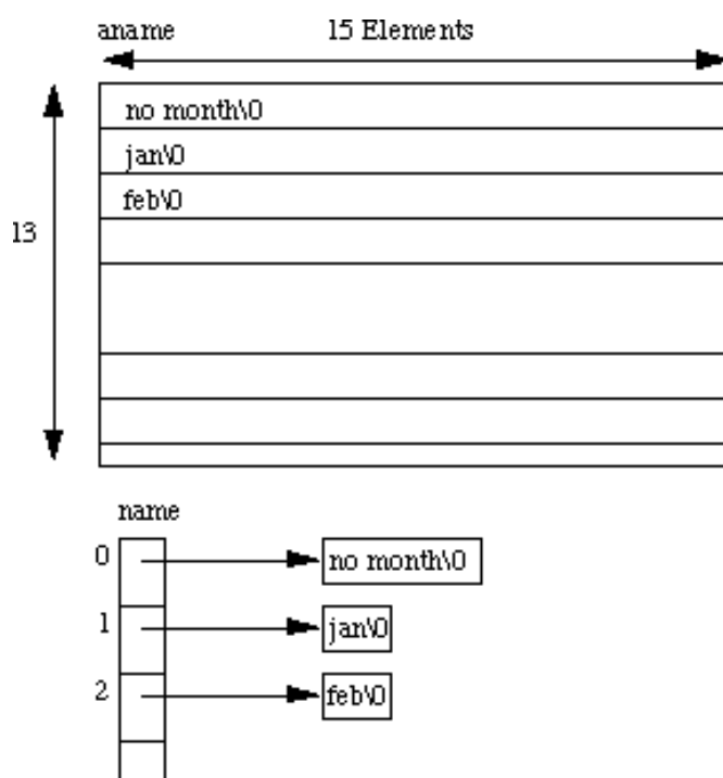
Figure 5.5: 2D Arrays and Arrays of Pointers
