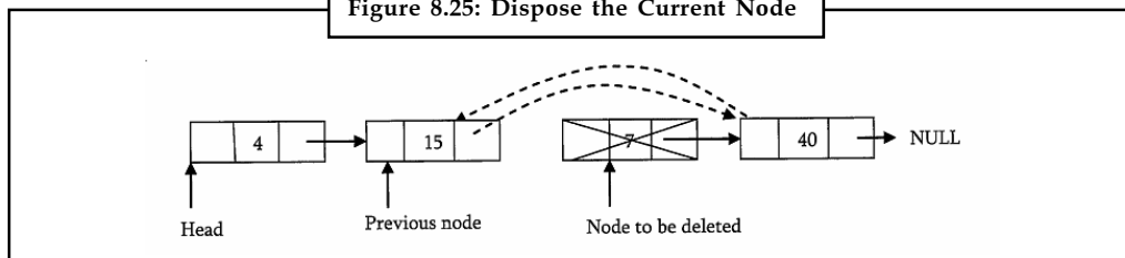
Figure 8.25: Dispose the Current Node
