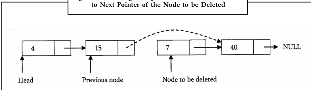
Figure 8.11: Change the previous Nodes Next Pointer to Next Pointer of the Node to be Deleted
