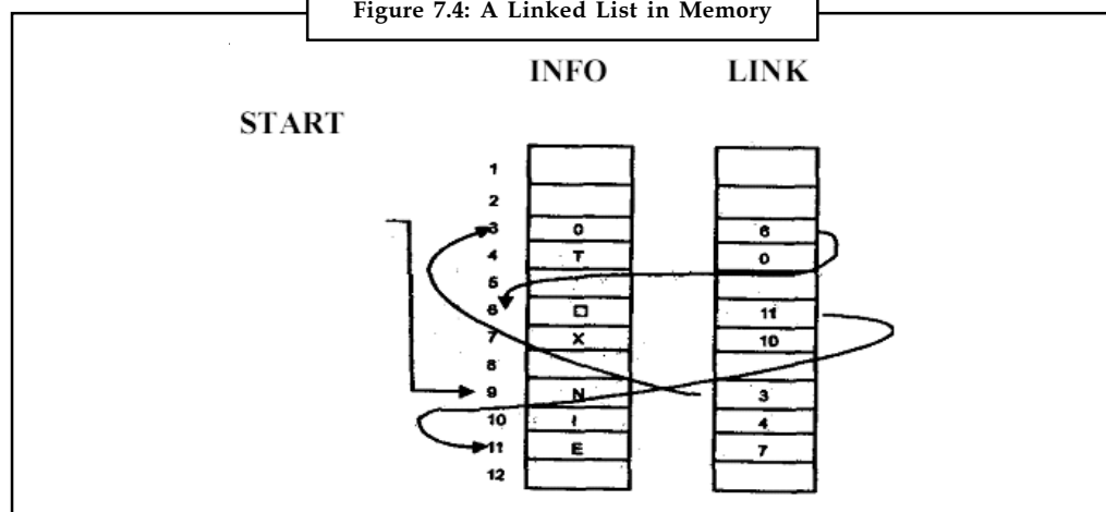
Figure 7.4: A Linked List in Memory
