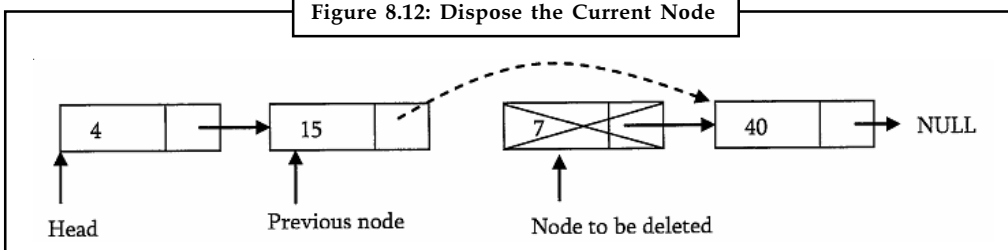
Figure 8.12: Dispose the Current Node
