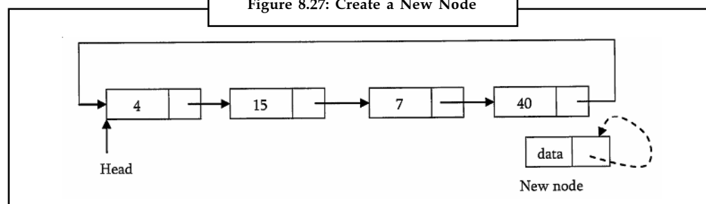
Figure 8.27: Create a New Node
