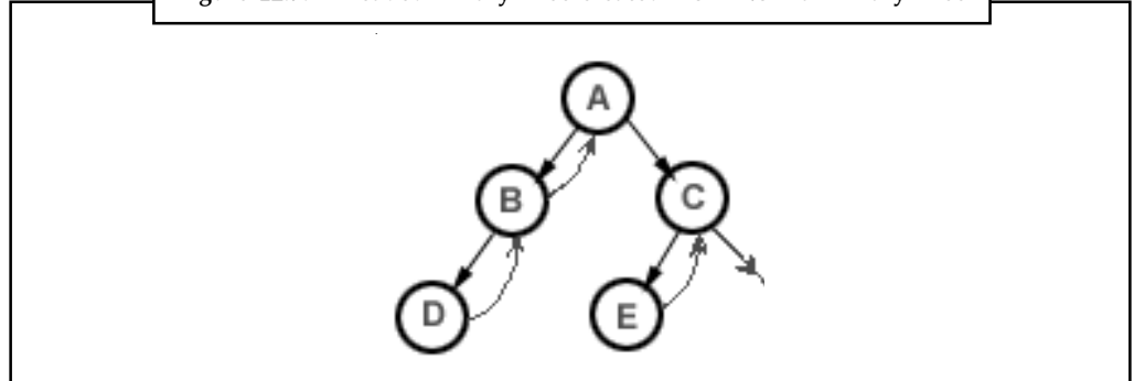
Figure 12.9: Threaded Binary Tree created from Normal Binary Tree
