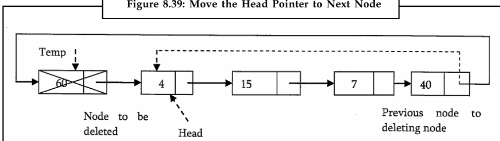
Figure 8.39: Move the Head Pointer to Next Node
