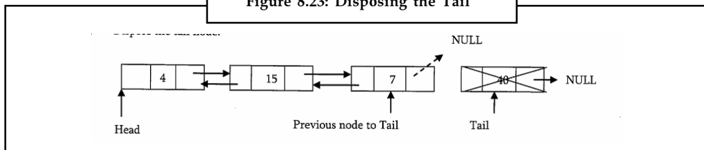
Figure 8.23: Disposing the Tail
