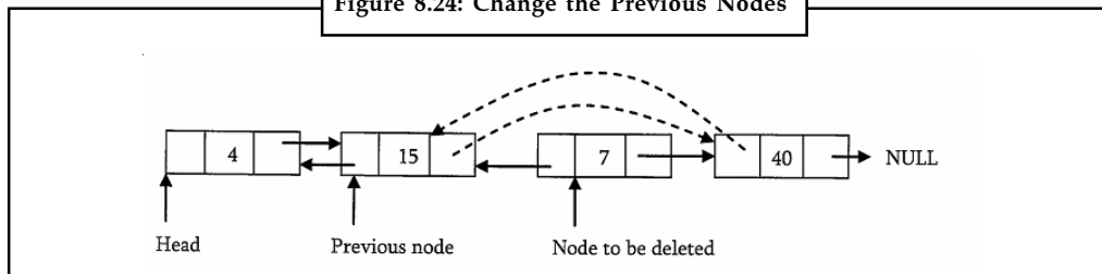
Figure 8.24: Change the Previous Nodes
