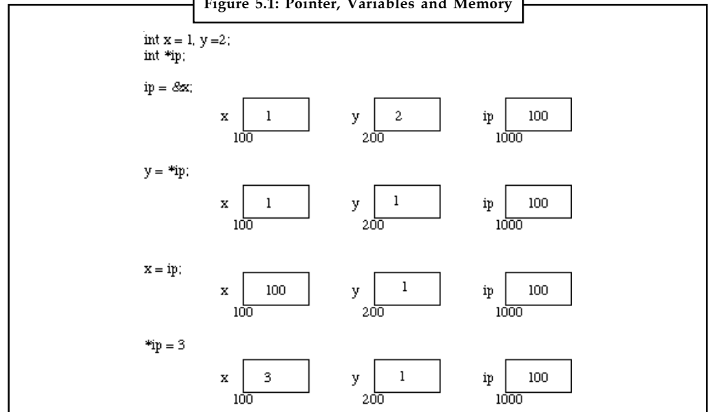
Figure 5.1: Pointer, Variables and Memory
