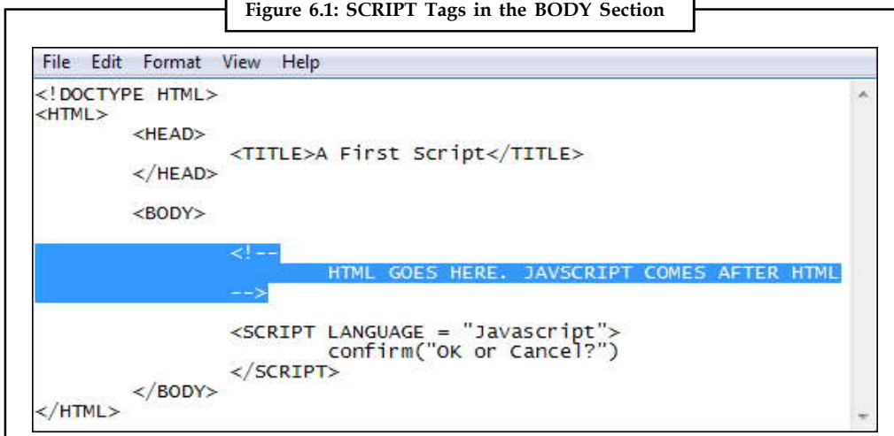
Figure 6.1: SCRIPT Tags in the BODY Section
