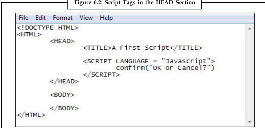
Figure 6.2: Script Tags in the HEAD Section
