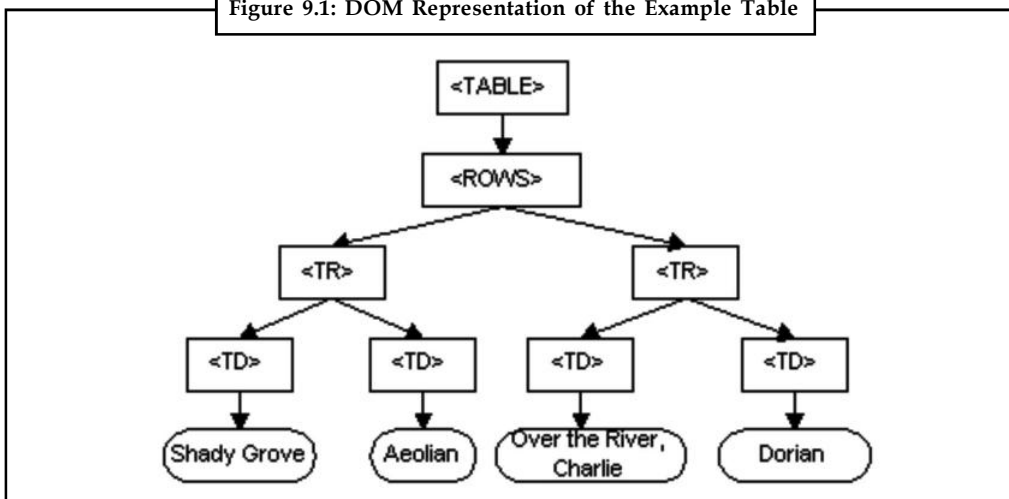
Figure 9.1: DOM Representation of the Example Table
