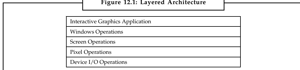
Figure 12.1: Layered Architecture
