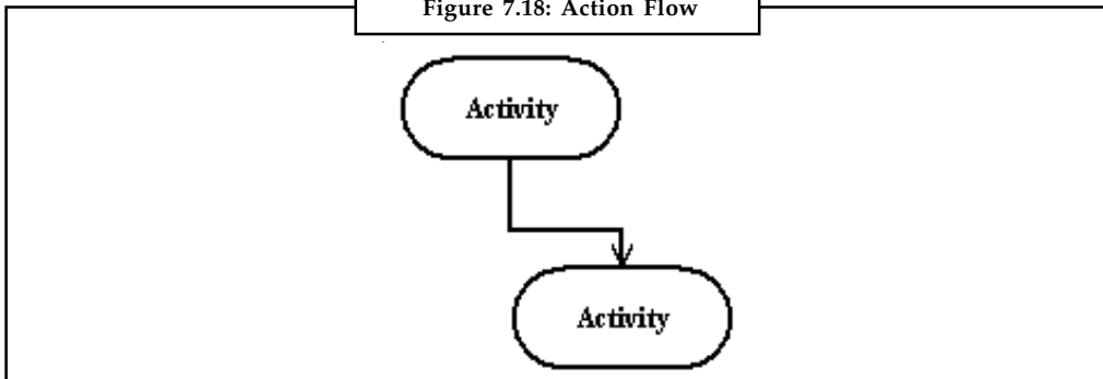
Figure 7.18: Action Flow
