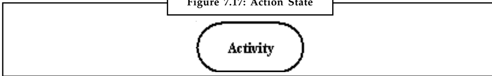
Figure 7.17: Action State
