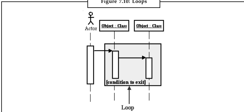
Figure 7.10: Loops
