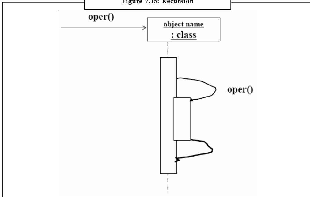
Figure 7.15: Recursion
