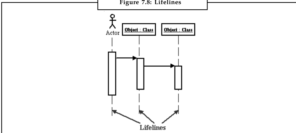
Figure 7.8: Lifelines
