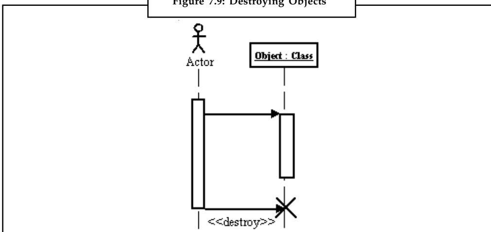
Figure 7.9: Destroying Objects
