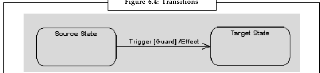
Figure 6.4: Transitions
