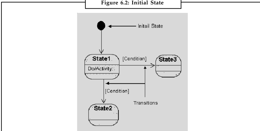
Figure 6.2: Initial State
