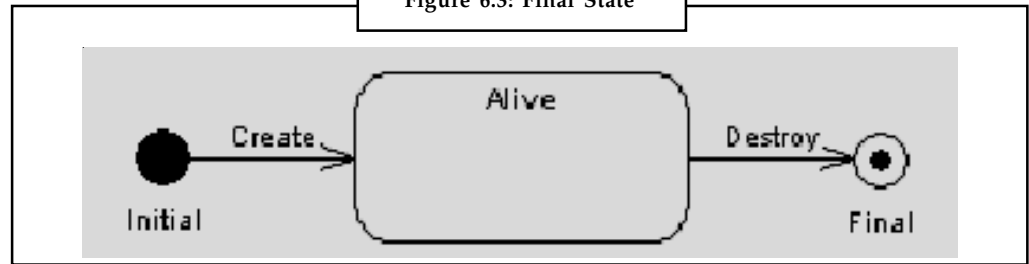
Figure 6.3: Final State
