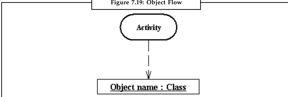
Figure 7.19: Object Flow
