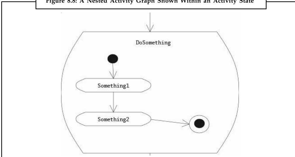
Figure 8.8: A Nested Activity Graph Shown Within an Activity State
