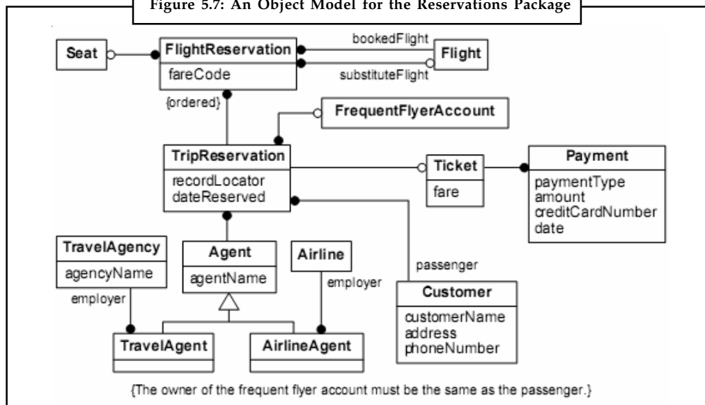
Figure 5.7: An Object Model for the Reservations Package
