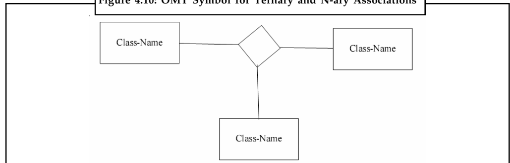
Figure 4.10: OMT Symbol for Ternary and N-ary Associations
