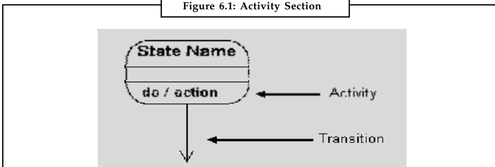
Figure 6.1: Activity Section
