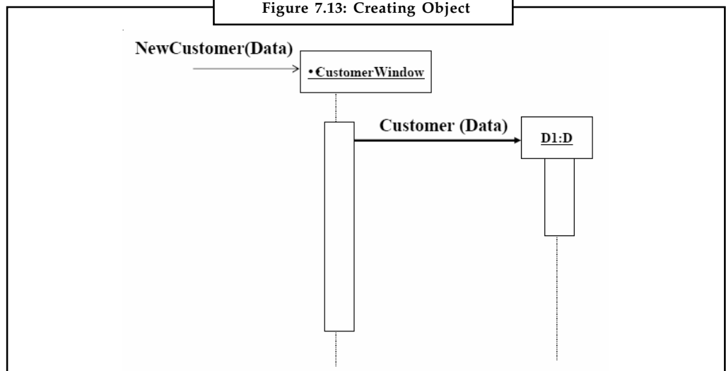
Figure 7.13: Creating Object
