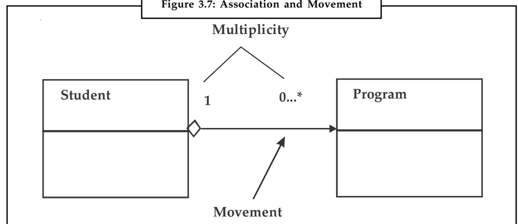
Figure 3.7: Association and Movement
