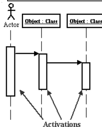
Figure 7.7: Activations
